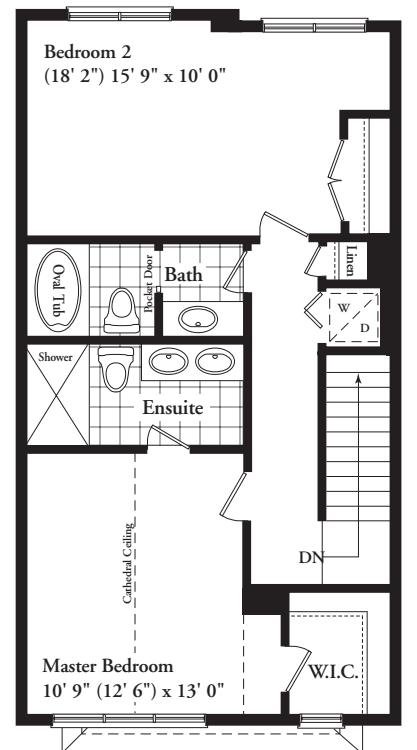
OPTIONAL SECOND FLOOR PLAN
