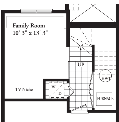
OPTIONAL GROUND FLOOR PLAN 2
