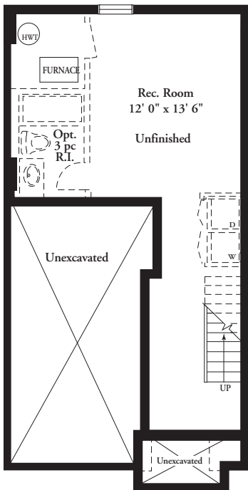
BASEMENT FLOOR PLAN (OPTIONAL FINISHED LAYOUT DOTTED)
